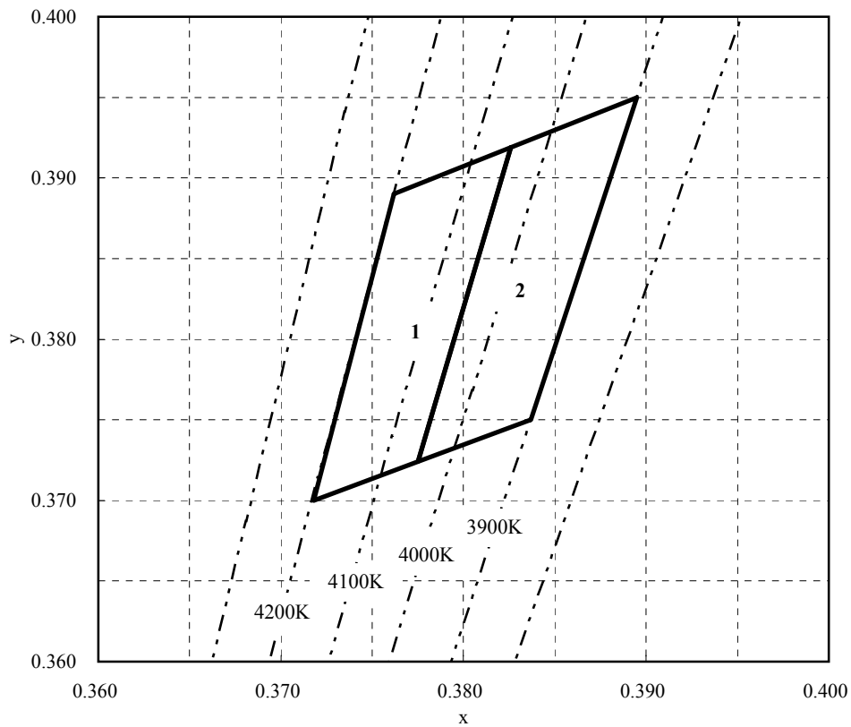
Chromaticity Diagram
